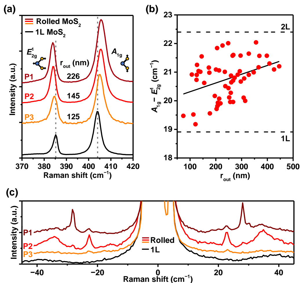
Figure 4. (a) Raman spectra of the \text{MoS}_2 nanoscroll measured at Spots P1, P2, and P3 indicated in Figure 1a. r_{\text{out}} estimated for each spot is indicated. The Raman spectrum of \text{MoS}_2 monolayer is also shown for reference. (b) Frequency difference between E_{2g}^1 and A_{1g} modes as a function of r_{\text{out}} estimated for 56 different spots on 15 different \text{MoS}_2 nanoscrolls. The solid line is the fitted slope. (c) Low-frequency ( \leq 45 \text{ cm}^{-1} ) Raman spectra of \text{MoS}_2 monolayer and the \text{MoS}_2 nanoscroll, measured at Spots P1, P2 and P3.
