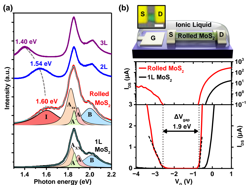
Figure 2. (a) PL spectrum of MoS 2 nanoscroll (red) presented along with PL spectra of mono- (black), bi- (blue) and trilayer (purple) MoS 2 . Multipeak Lorentzian fittings are produced for the PL spectra of the scrolled MoS 2 and MoS 2 monolayer, and cyan solid lines represent fitted curves. (b) Schematic diagram of the ionic-liquid-gated transistor and an optical image of scrolled MoS 2 transistor. White scale bar indicates 1 \mu m (top). Transfer characteristics of MoS 2 nanoscroll and MoS 2 monolayer transistors presented in semilogarithmic (middle) and in linear scales (bottom).
