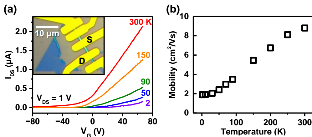
Figure 3. (a) Transfer characteristics of a MoS 2 nanoscroll FET, measured at different temperatures between 2 and 300 K. Inset presents an optical image of the transistor. (b) Estimated field-effect electron mobility of the MoS 2 nanoscroll as a function of temperature.
