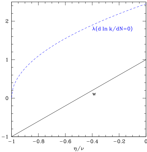
Fig. 1. The ratio \eta/\nu of the anomalous dimensions of the RG flow variables determines the cosmological fixed point for the third critical point. The solid black curve shows the dark energy equation of state dominating the future cosmic expansion, while the blue dashed curve shows the value of \lambda for which the RG flow freezes. Runaway potentials such as inverse power laws give \lambda = 0 and so w = -1 . (For interpretation of the references to color in this figure legend, the reader is referred to the web version of this Letter.)
